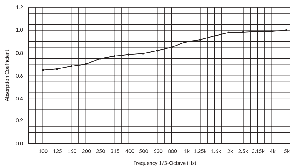
Sound absorption coefficient diagram
